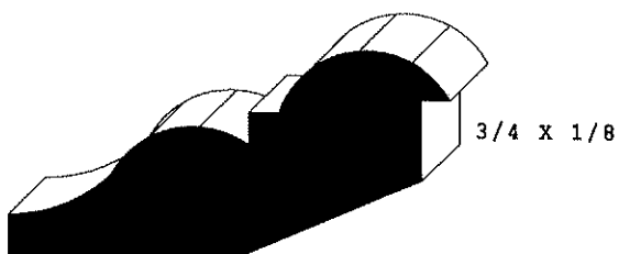
RBP #557 (1 X 2-1/16)
